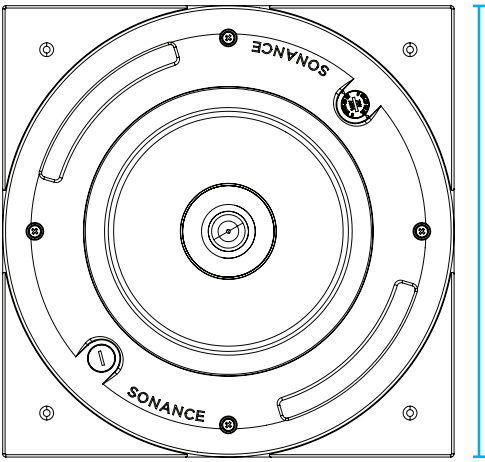
Square Adapter Front 11.07" (281.1mm)
